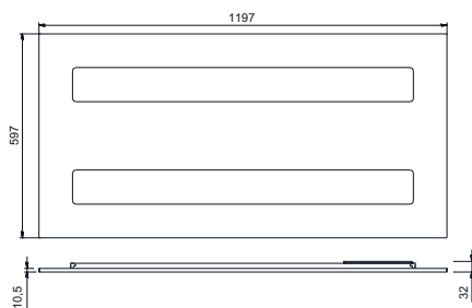
SmartBright Troffer RC098V
